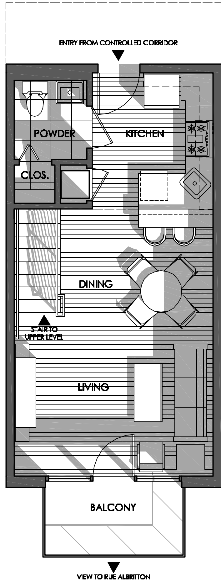
SPLIT-LEVEL UNIT (LOWER LEVEL)
